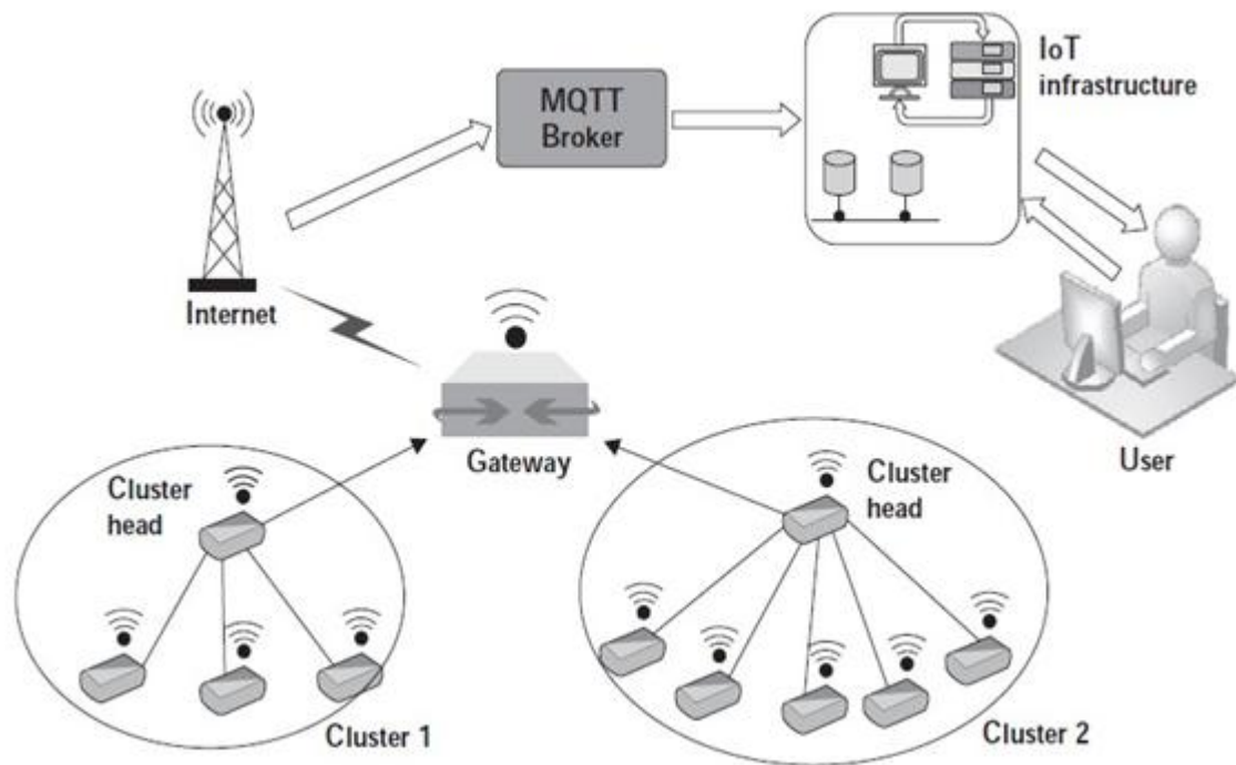
Figure 4: System Architecture
